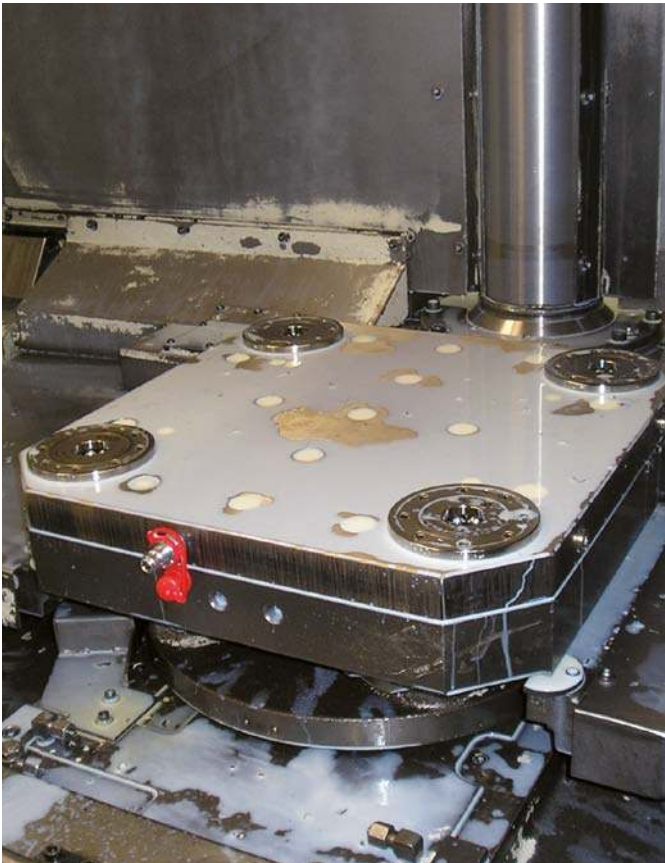
The interior of the clamping module is completely sealed. This means that the system is optimally protected against liquids and dirt.
