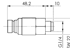
427856 connector
