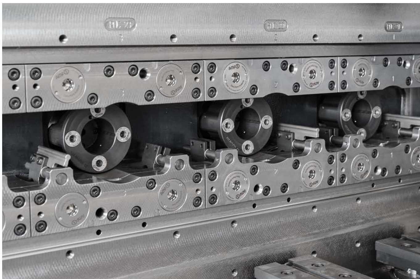
Each receptacle is equipped with four zero-point clamping modules. Thanks to the compact design, the clamping modules can be screwed in easily and flush.
