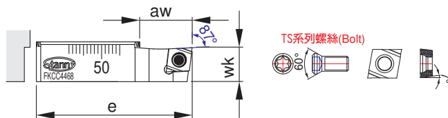
菱形精搪孔反搪刀座 Rhombus Reverse Cutting Insert Holder
