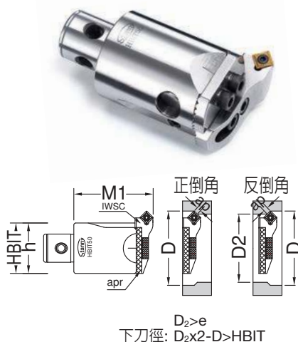
45°正反倒角粗搪頭系統組合 Body and 45° Chamfer Cutting Insert Holder
