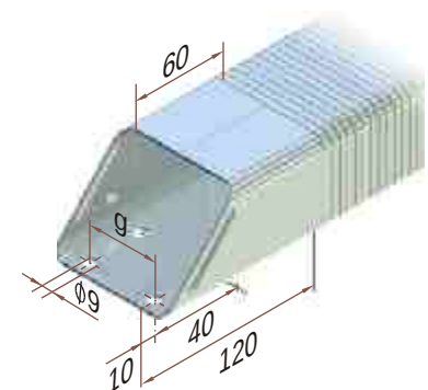
scoop bracket
