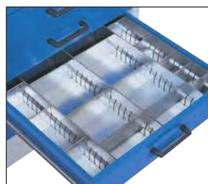
Drawer partitioning
